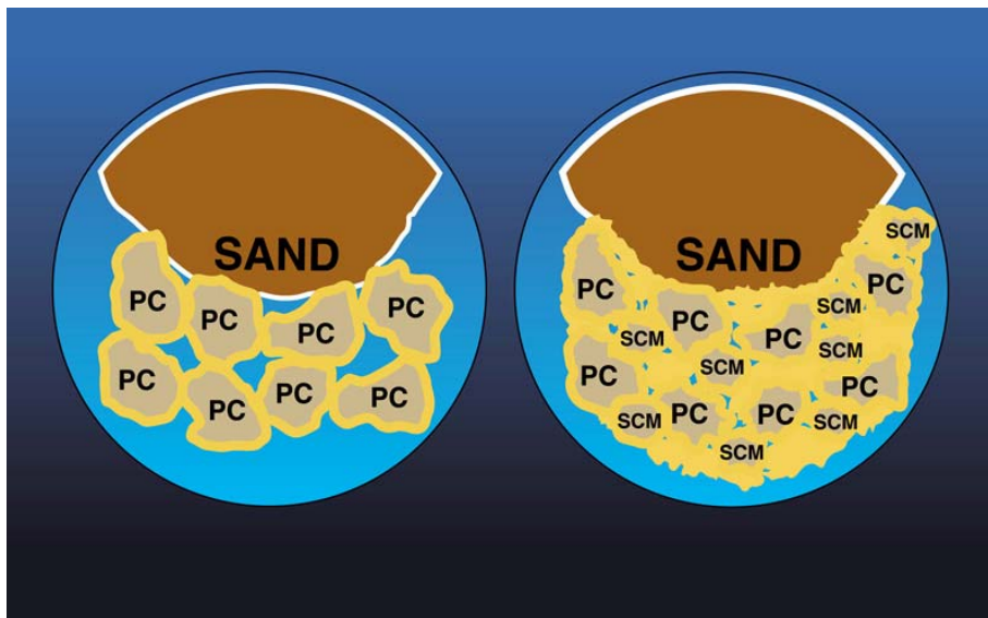
Figure 1. (Left) When ordinary portland cement (PC) hydrates, C-S-H is formed (yellow); this glue holds concrete together. However, gaps in this glue provide pathways for moisture to penetrate and reduce strength. (Right) When supplementary cementitious materials (SCM) are added, particles pack more tightly within the voids and additional glue forms from the SCM hydration process. With fewer voids, the concrete is less permeable and stronger.
