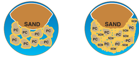
Figure 1: When ordinary portland cement (PC) hydrates (left), C-S-H is formed (shown in yellow); this glue holds the concrete together. However, gaps in this glue provide pathways for moisture to penetrate and reduce strength. When supplementary cementitious materials (SCM) are added (right), particles pack more tightly within the voids and additional glue forms from the SCM hydration process. With fewer voids, the concrete is less permeable and stronger.
