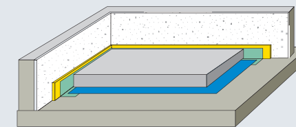
Separation layer system
