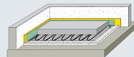
Electrical heating system
